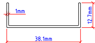
U-Channel Scale 1:1
