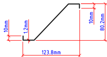
2544C Scale 1:4
