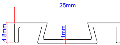
SJ258 (Trimming)
