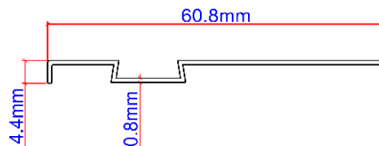
SJ259 (Skirting)
