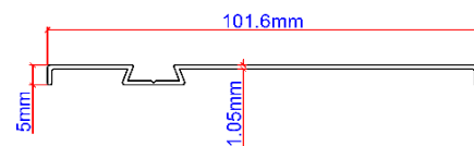
FF806B (Skirting)
