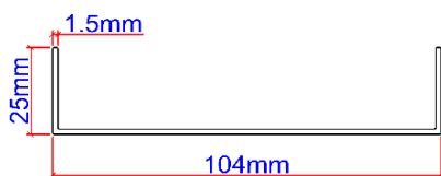
CK4448 (U-Channel)
