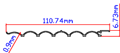
BJ051 (4" Spandrel)
